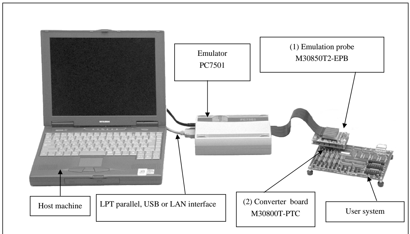
Figure 1.1 System configuration
